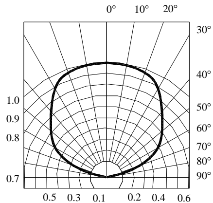
Radiation Diagram
